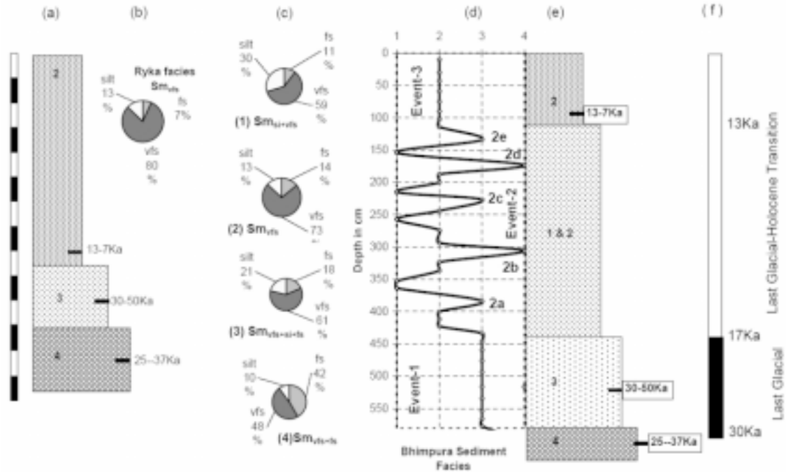
Figure 2. Details of litho facies from Bhimpura and Rayka. a) Litholog of Rayka section along with luminescence ages (Juyal et al. 2000); b) Sediment facies at Rayka section; c) Sediment facies at Bhimpura, namely: 1) Massive, unstratified silt + Very fine sand + silt ( Sm_{si+vfs} ), 2) Massive unstratified very fine sand ( Sm_{vfs} ) 3) Massive unstratified very Fine Sand + silt + fine sand ( Sm_{vfs+si+fs} ) and 4) Massive unstratified very fine sand + fine sand facies ( Sm_{vfs+fs} ). d) Change in facies at Bhimpura decoded using cluster analysis. X-axis represents sediment facies while Y-axis represents depth. Events and sub-events are separately marked. e) Litholog of Bhimpura section (0-580 cm). The number within litholog represents facies code, while the number in rectangle represent interpolated ages of individual sediment facies. f) Age model for Bhimpura section.
