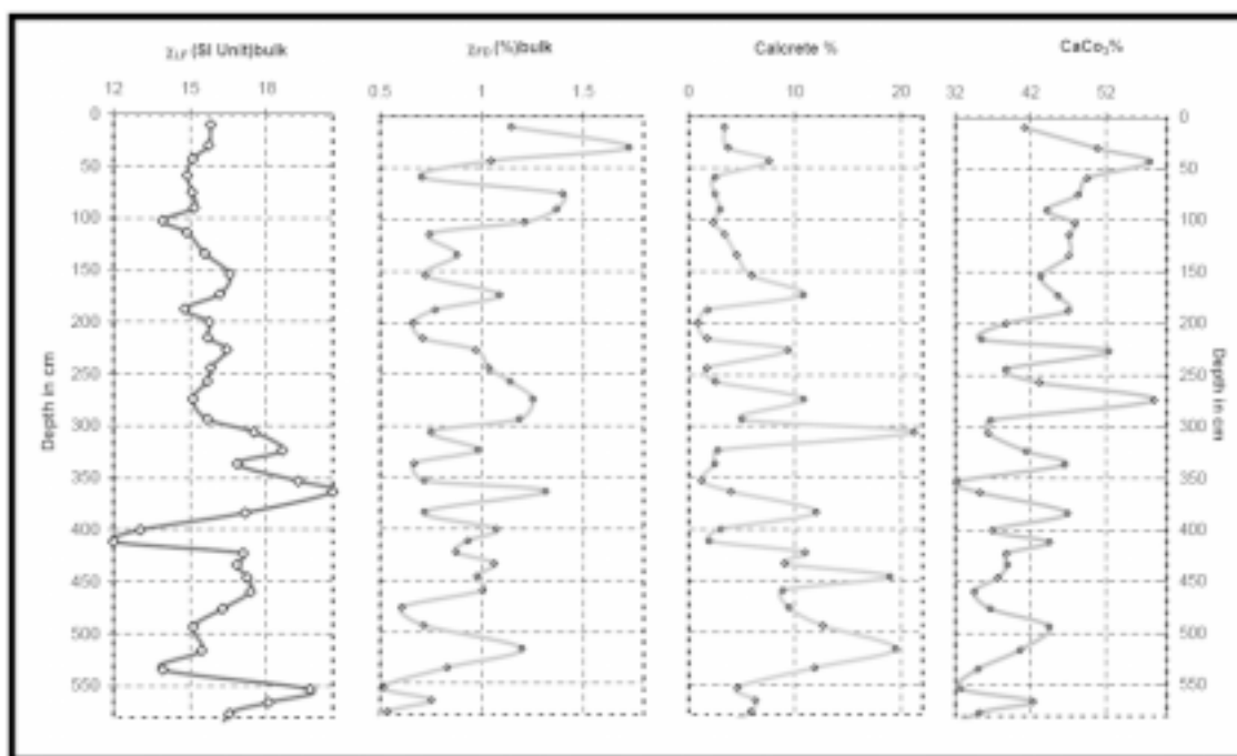
Figure 4. Climate sensitive allogenic and authigenic proxies namely magnetic susceptibility ( \chi_{\text{LF}} bulk, and \chi_{\text{FD}} % bulk), calcrete percentage and carbonate percentage.
