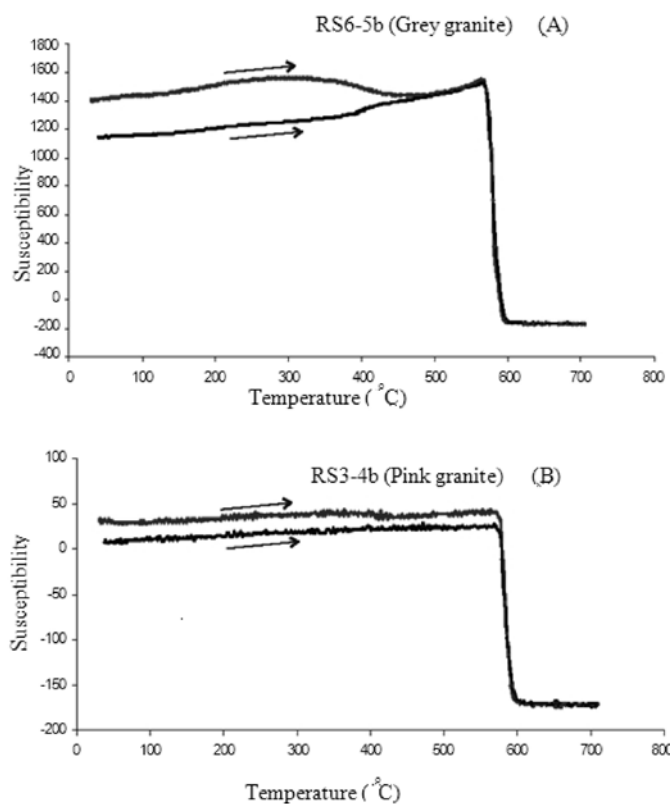
Figure 4. K-T curves of A: Grey granite, B: Pink granite
