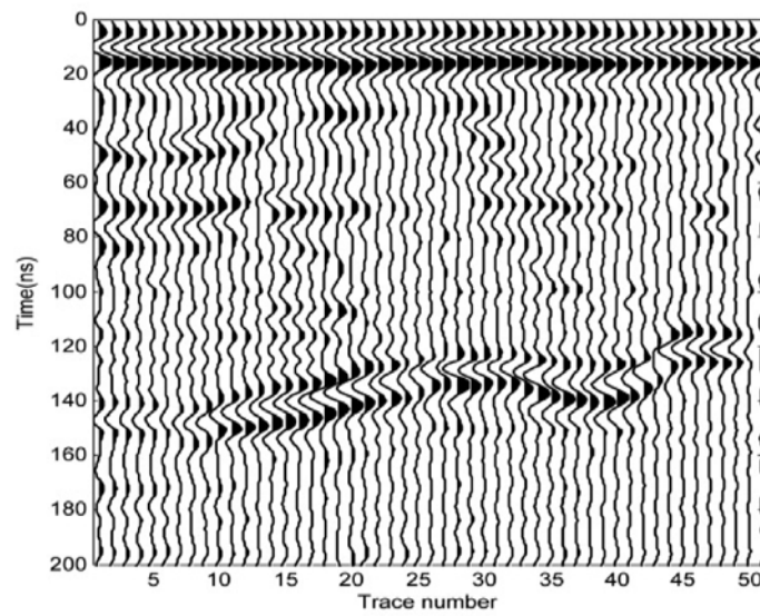
Figure 3. GPR section.
