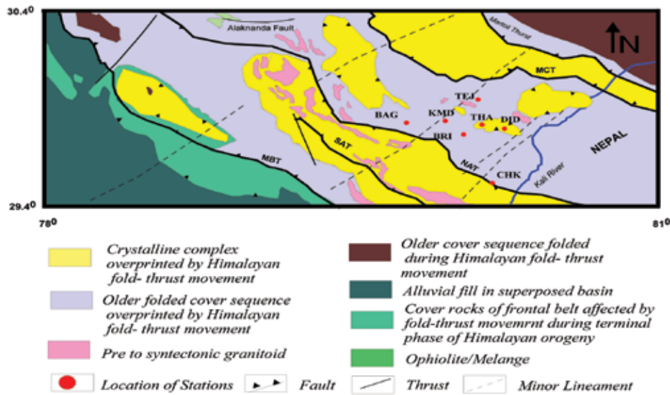
Figure 1. The present area of study belongs to the Kumaon and Garhwal Himalayas, India. MBT = Main Boundary Thrust, MCT = Main Central Thrust, and NAT = North Almora Thrust. Red circles show the location of the stations. Source of the tectonics and geology of the region is as per GSI (2000).
